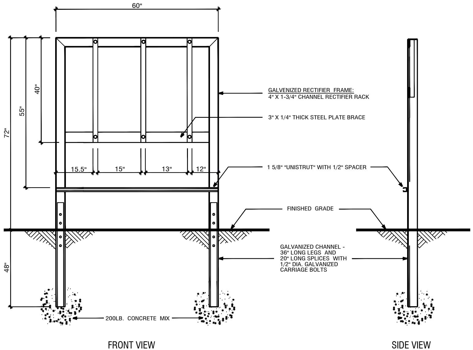
TYPICAL R-0 RECTIFIER RACK
